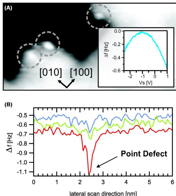
Fig. 5 (A) NC-AFM image of an MgO step edge on Ag(001); point defects are highlighted. A frequency shift vs. bias voltage spectroscopy curve acquired on a defect is presented in the inset, facilitating the determination of the associated charge state. (B) Frequency shift data recorded along a horizontal line passing over a point defect at three different tip-sample distances separated by 0.5 Å, with the red curve corresponding to the smallest separation. Negative frequency shift values are detected at the defect site, indicative of attractive tip-sample interactions. Reprinted with permission from König, T., et al. (2009) J. Am. Chem. Soc. 131, 17544–17545 (A) and König, T., et al. (2010) ACS Nano 4, 2510–2514 (B). Copyright (2009) and (2010) American Chemical Society.
